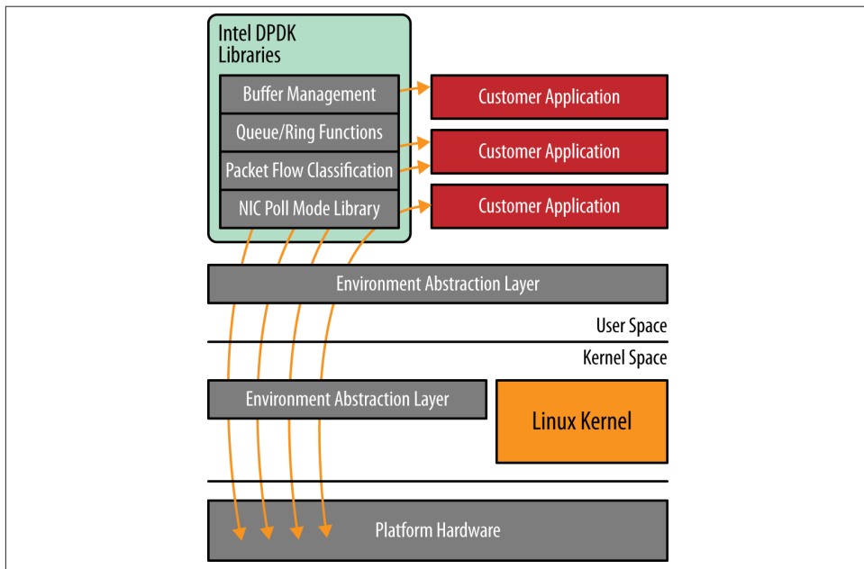
Figure 7-3. Intel DPDK
