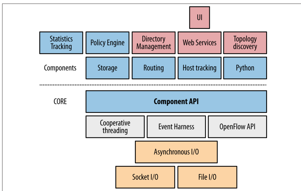
Figure 4-10. NOX architecture
