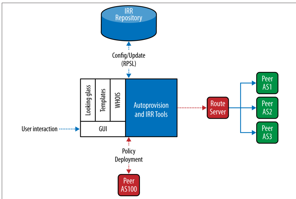
Figure 2-17. IIR and route server interconnection
