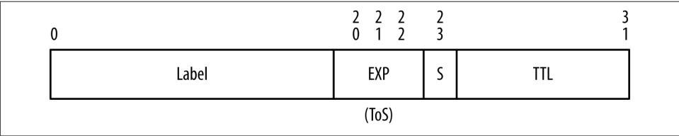
Figure 2-13. MPLS label
