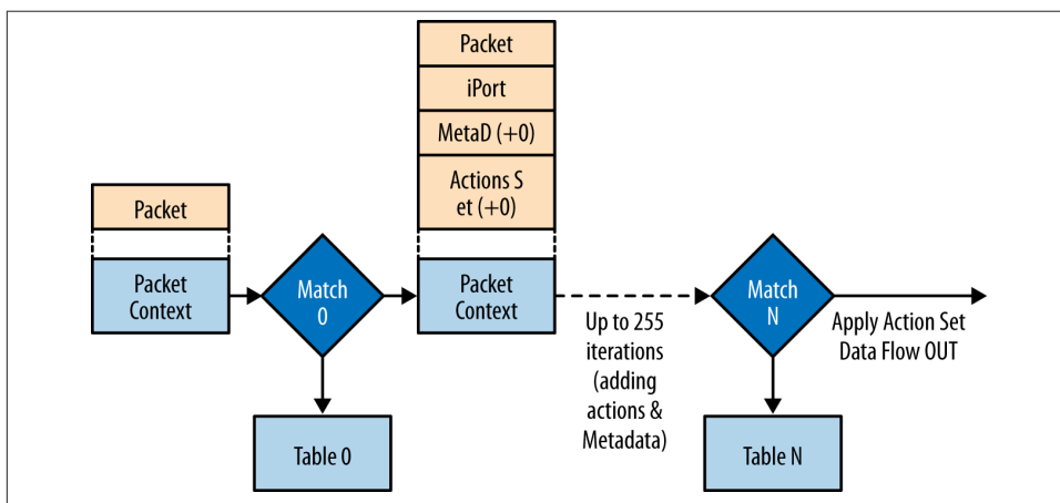
Figure 3-4. The post OpenFlow pipeline model in version 1.1 and beyond (very complex—combinations complexity O(n! \cdot a(2^l)) paths where n = number of tables, a = number of actions and l = width of match fields)
