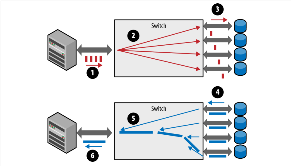
Figure 9-7. Incast/micro-burst
