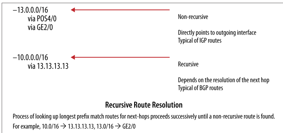
Figure 2-11. Route recursion
