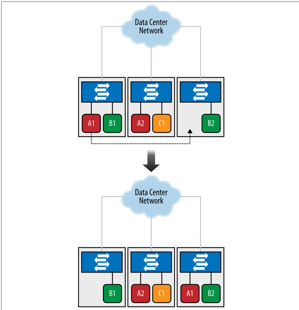
Figure 6-12. VM migration
