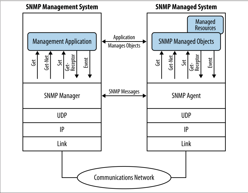
Figure 5-4. The basics of the SNMP Architecture are comprised of an SNMP Management system and an SNMP Managed System
