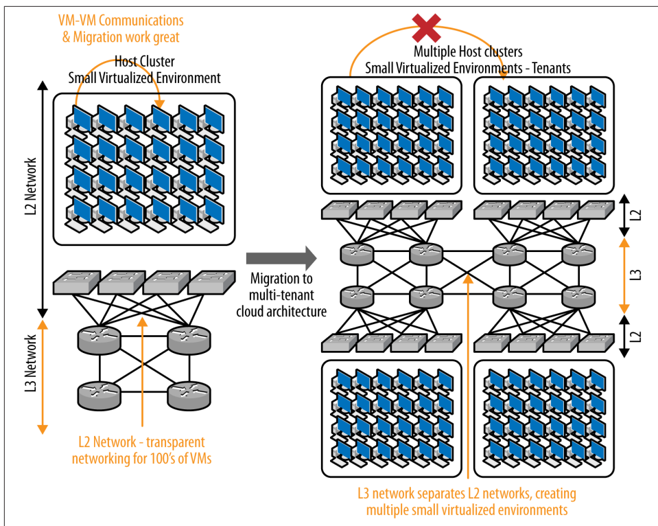
Figure 6-23. NVGRE overlay networks: enabling network scalability for a cloud infrastructure
